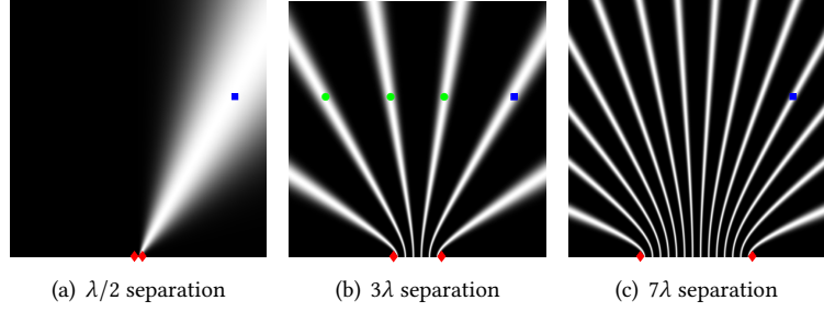
Fig. 3. Increasing inter-element separation will cause ambiguous angles of arrival. As the separation of two microphones (red diamond marker) increases, the beams become finer, but causing ambiguity (some examples are marked by green dots) in localizing the true sound source (blue square marker).
